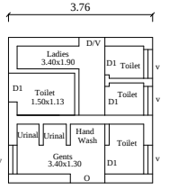
TOILET BLOCK PLAN
