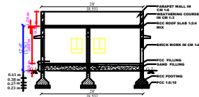
SECTION ON - AB
