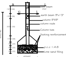
FOUNDATION DETAILS
