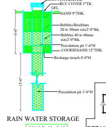
RAIN WATER STORAGE
