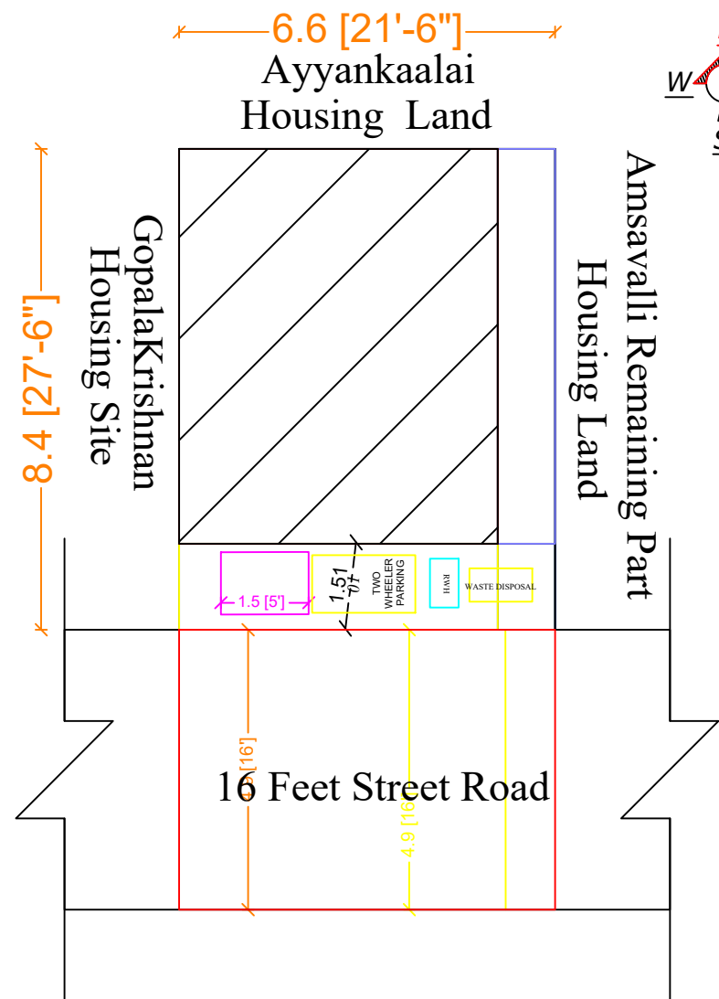
SITE PLAN / KEY PLAN PROPOSED NEW CONSTRUCTION
