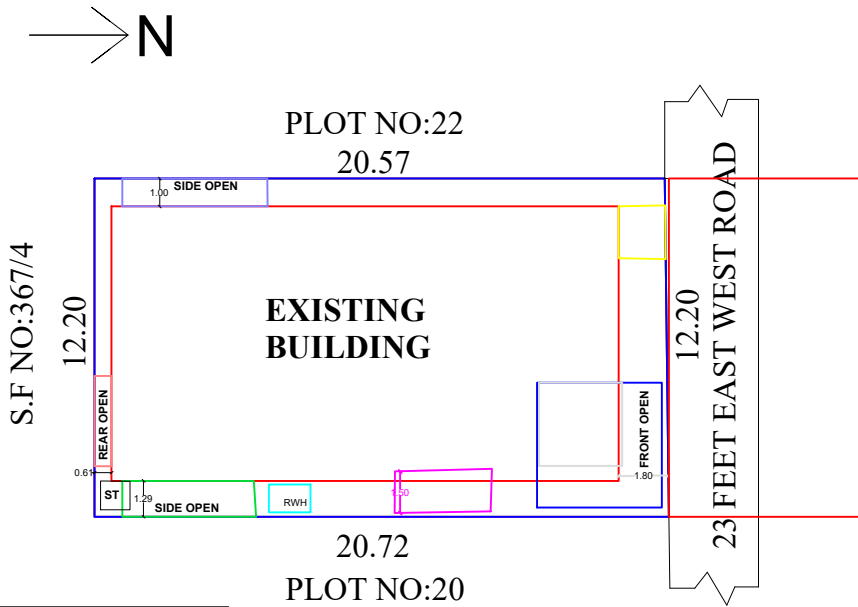
AREA DETAILS AREA DETAILS SQ.MT SQ.FT TOTAL PLOT AREA :- 252 2710 AREA OF THE EXT. GROUND FLOOR BUILDING 181.16 1949.99 AREA OF THE OPEN SPACE 70.84 760.01
