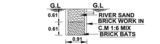
. SECTION ON RAIN WATER COLLECTION TUB .
