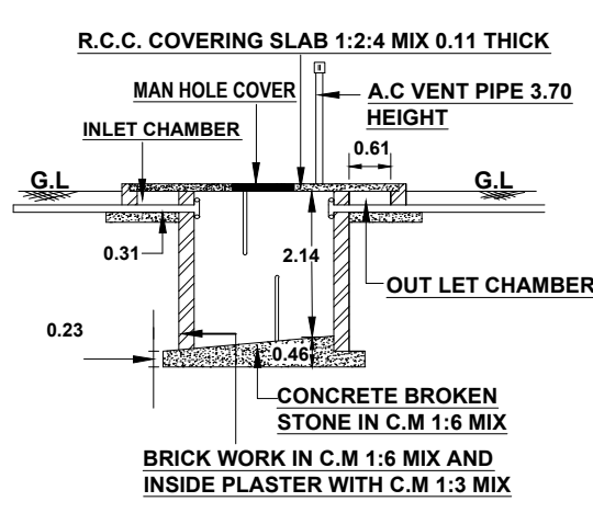
.SECTION ON SEPTIC TANK .
