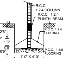
FOUNDATION DETAIL
