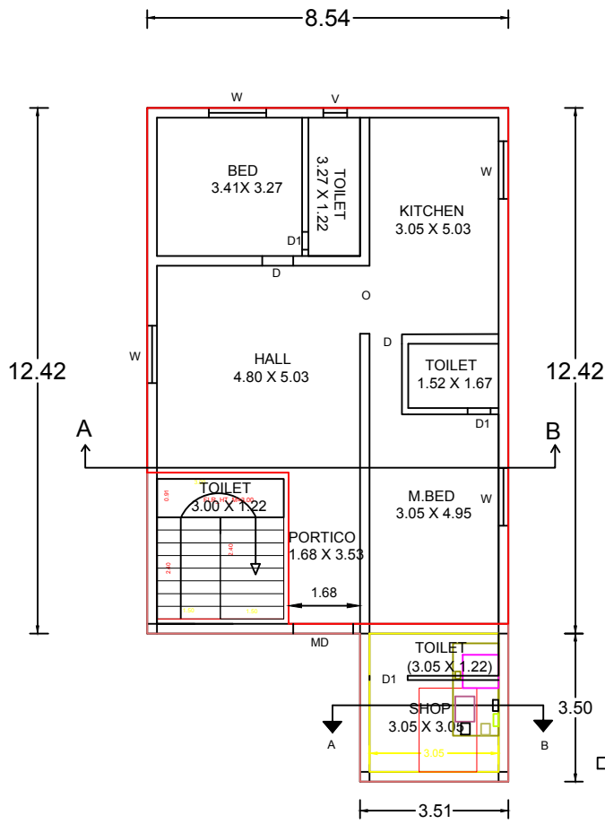
EXISTING & PROPOSED GROUND FLOOR PLAN
