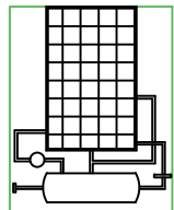
SOLAR SYSTEM
