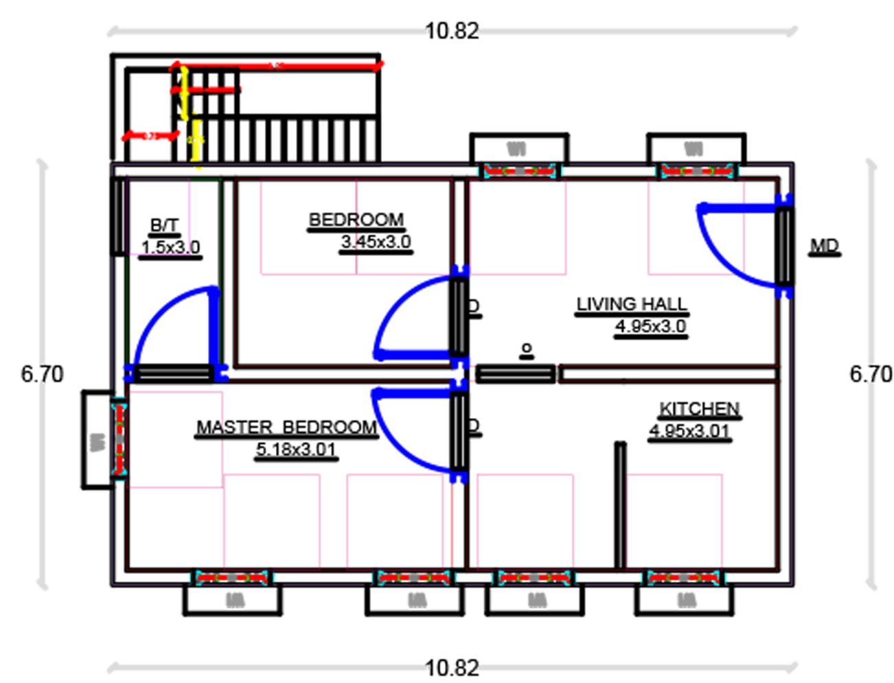
PRO GROUND FLOOR
