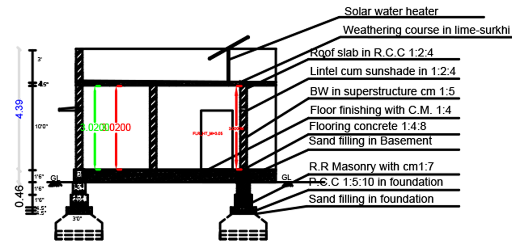
SECTION
