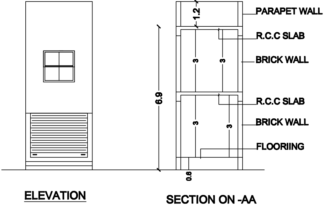
SECTION ON-AA
