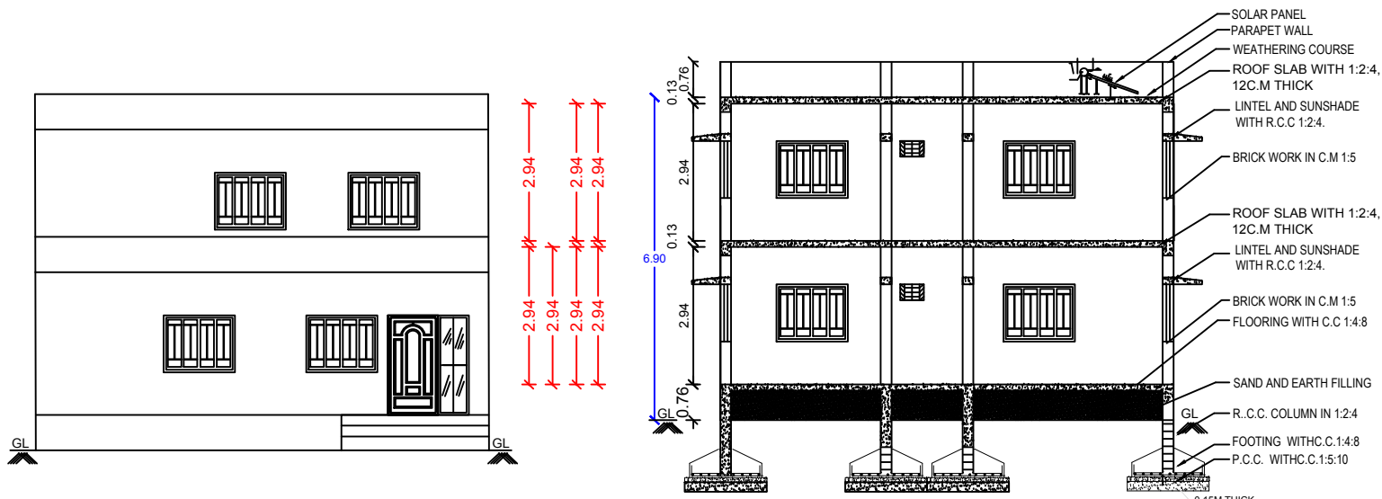
FRONT ELEVATION (EAST FACING)
