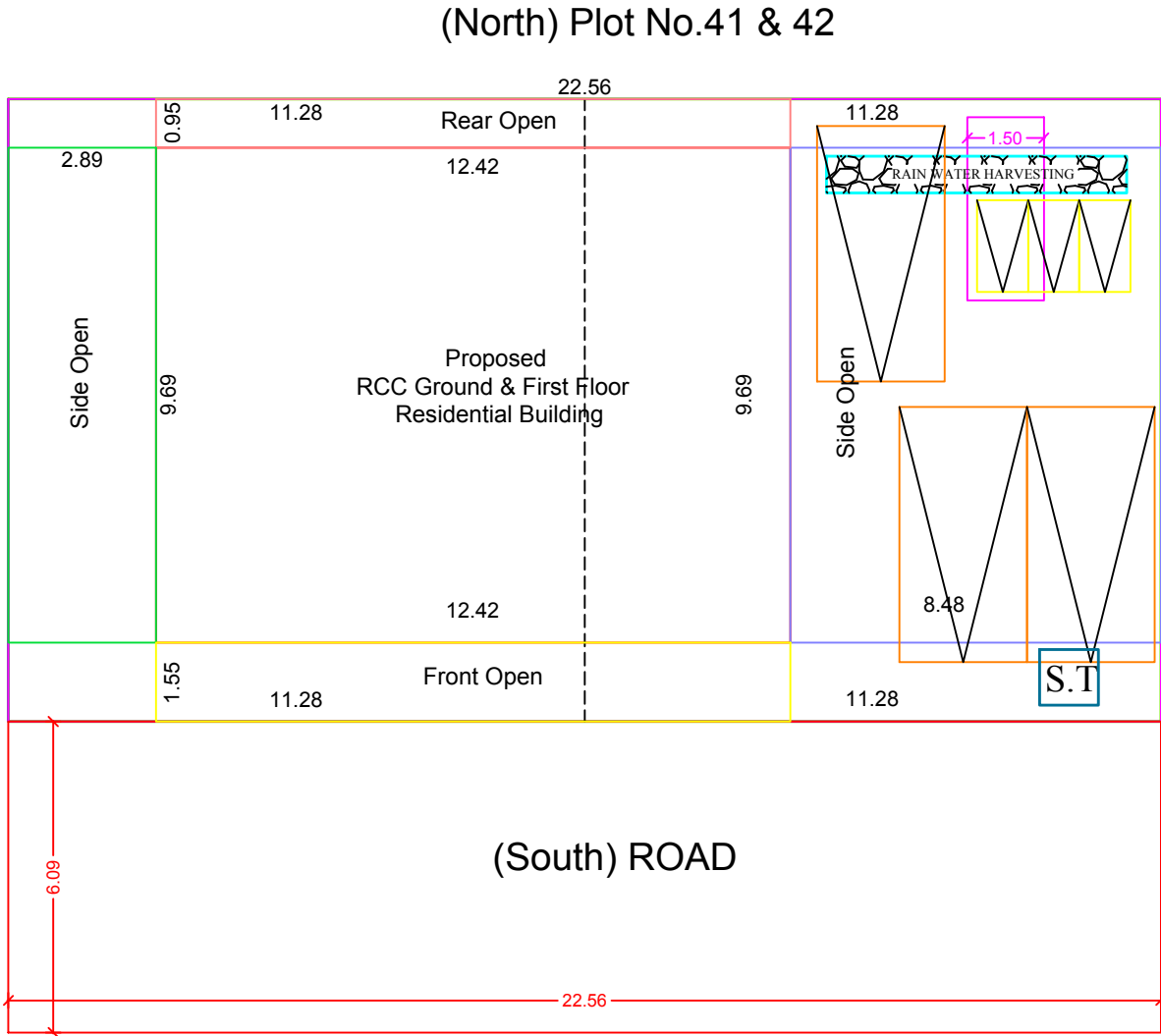
SITE PLAN
