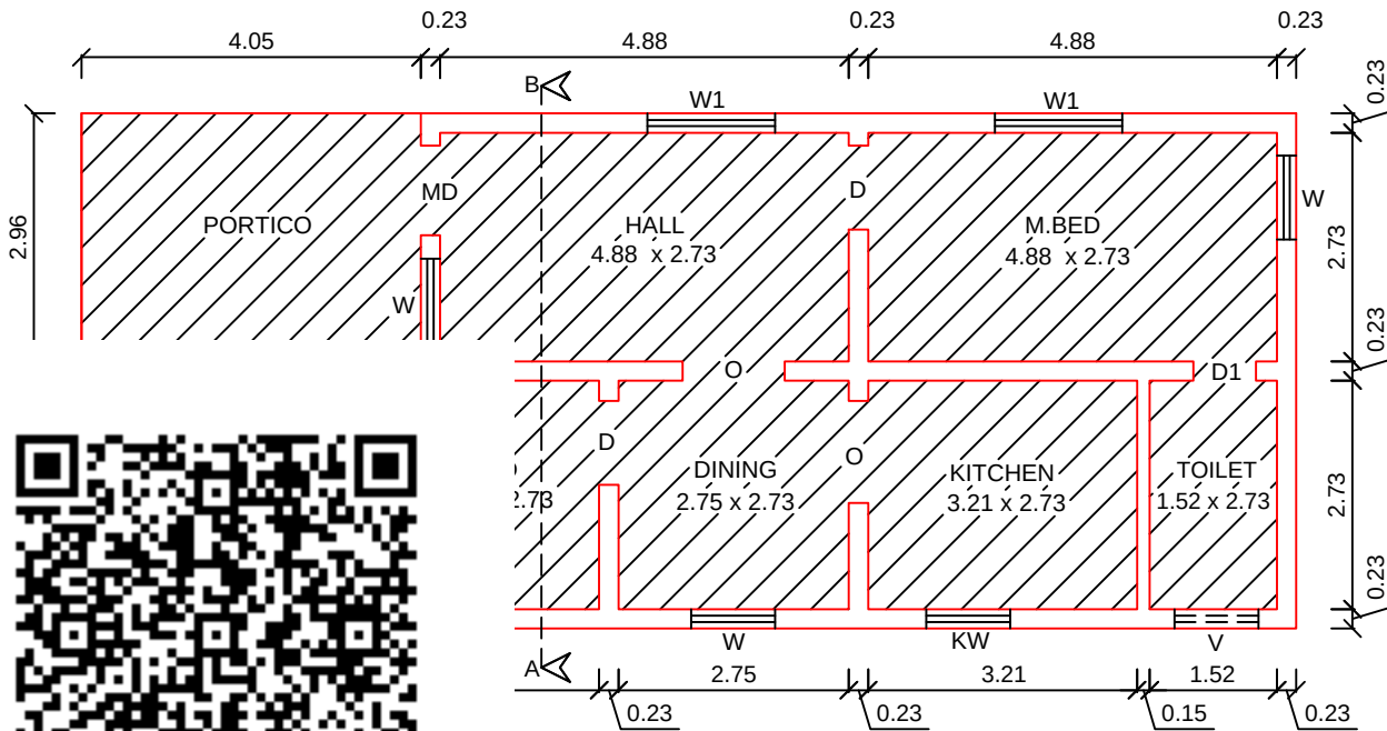
ROUND FLOOR PLAN
