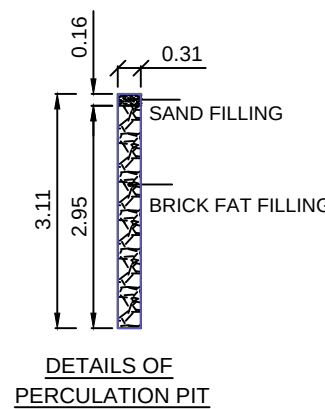
DETAILS OF PERCOLATION PIT
