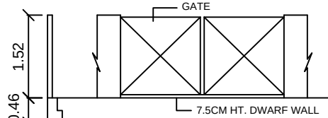
COMPOUND WALL WITH DWARF WALL DETAILS
