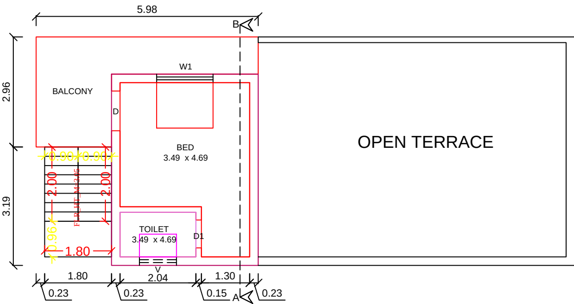
PRO.SECOND FLOOR PLAN
