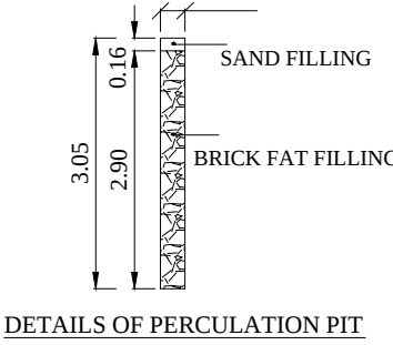
DETAILS OF PERCOLATION PIT
