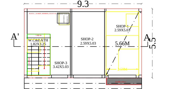
EXISTING APPROVAL GROUND FLOOR PLAN
