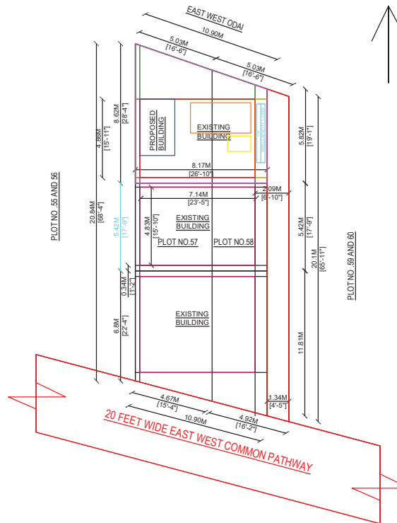
SITE PLAN
