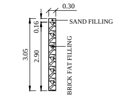
DETAILS OF PERCOLATION PIT
