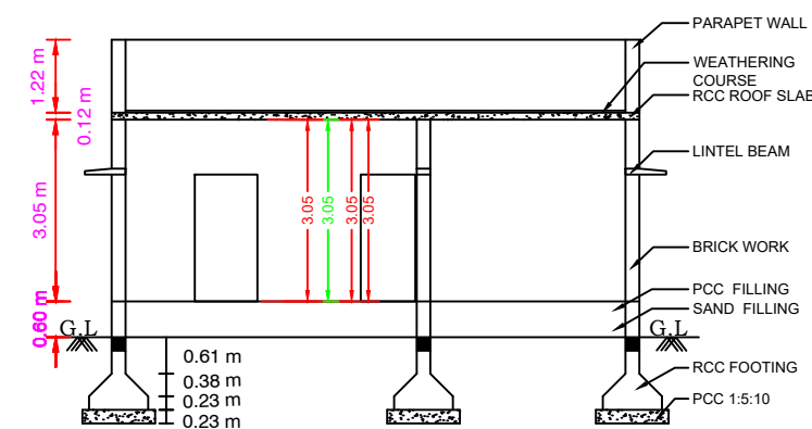
SECTION ON KA
