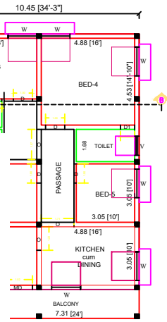
FLOOR PLAN
