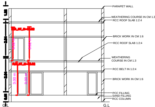
SECTION ON-AA&BB
