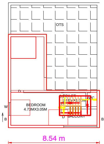
FIRST FLOOR(Pro.)
