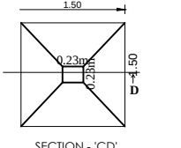
SECTION - 'CD'
