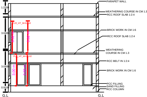
SECTION ON-AA&BB
