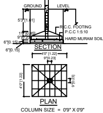
FOUNDATION DETAILS
