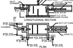
SEPTIC TANK:
