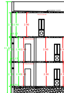
SECTION ON K-S
