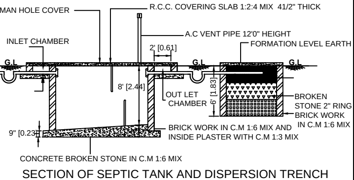
SECTION OF SEPTIC TANK AND DISPERSION TRENCH
