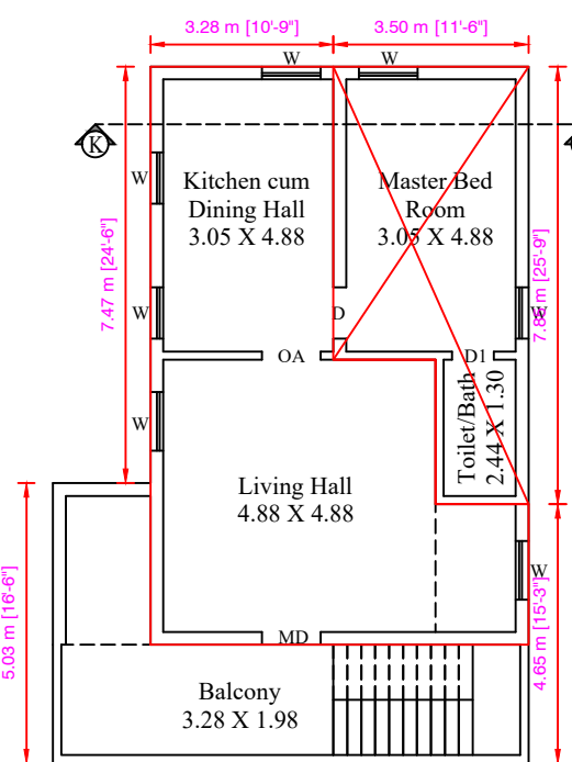
EXISTING & ADDITIONAL FIRST FLOOR PLAN
