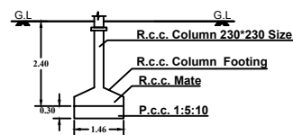
Foundation Details
