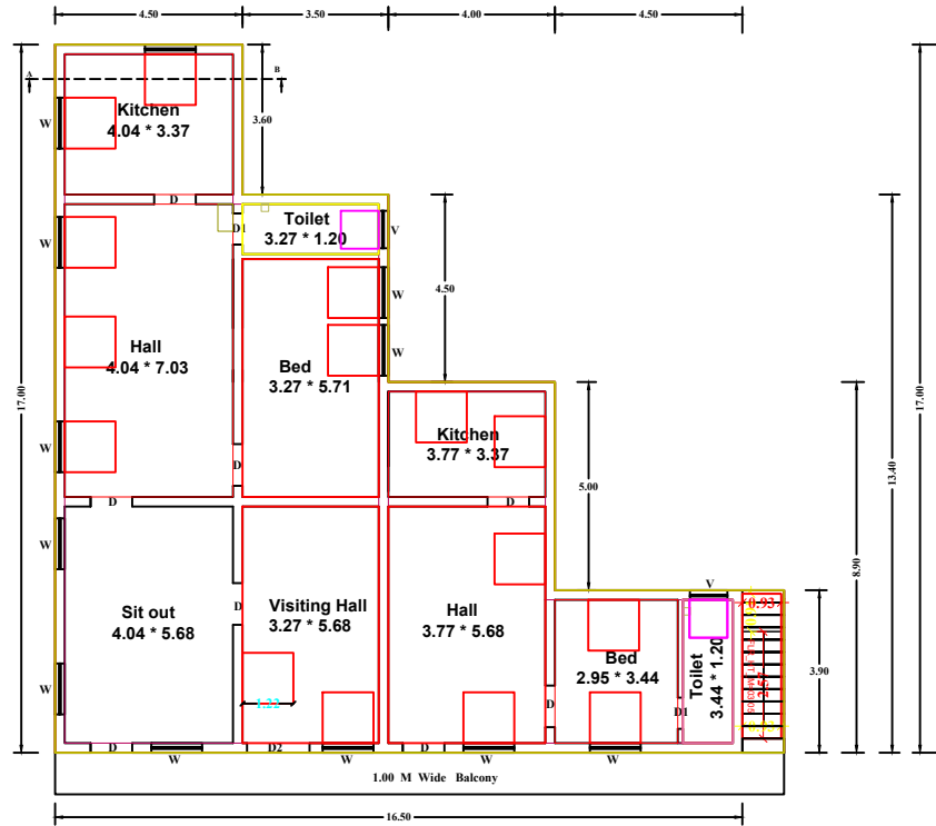
ADDITIONAL PROPOSED F.FLOOR RESIDENTIAL BUILDING
