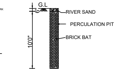
PERCOLATION PIT
