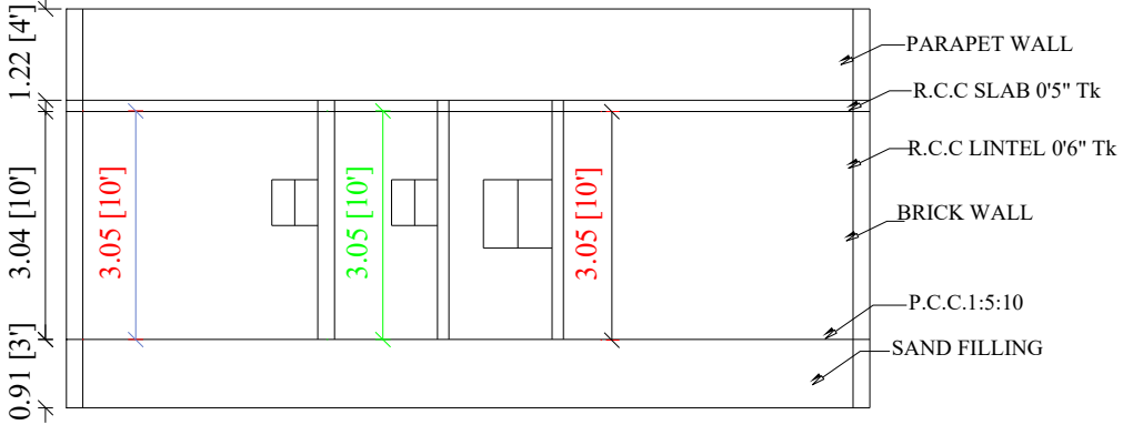
SECTION ON"AB"
