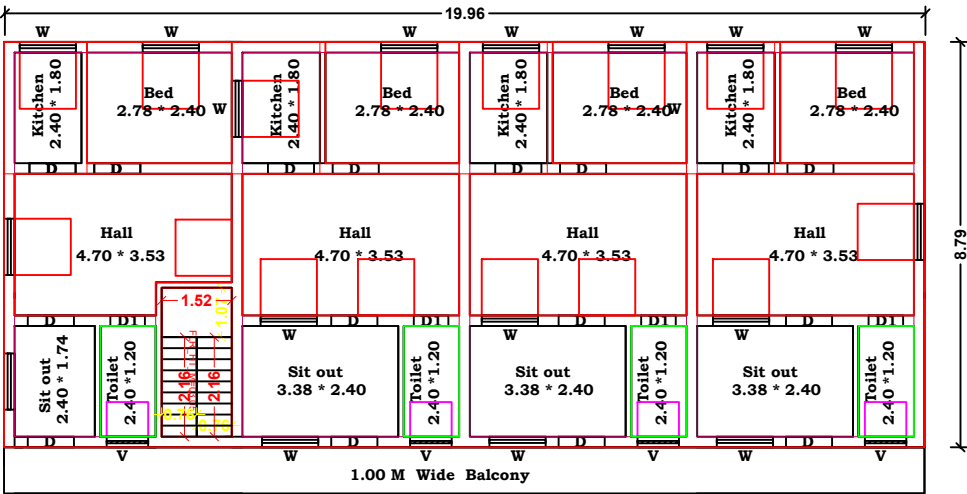
Revised First Floor Plan
