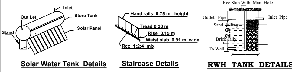
Solar Water Tank Details
