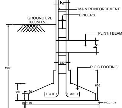
TYPICAL SECTION OF R.C.C COLUMN FOUNDATION
