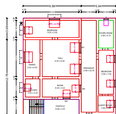
EXISTING GROUND FLOOR PLAN AND PROPOSED GROUND FLOOR PLAN (EAST FACING)
