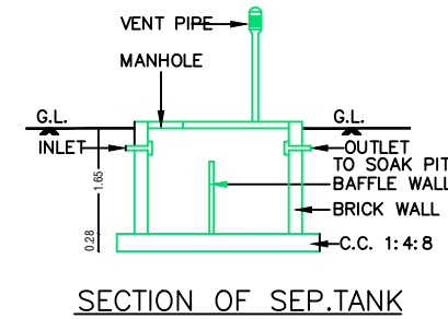
SECTION OF SEPT.TANK
