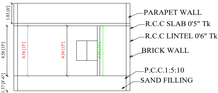
SECTION ON"AB"
