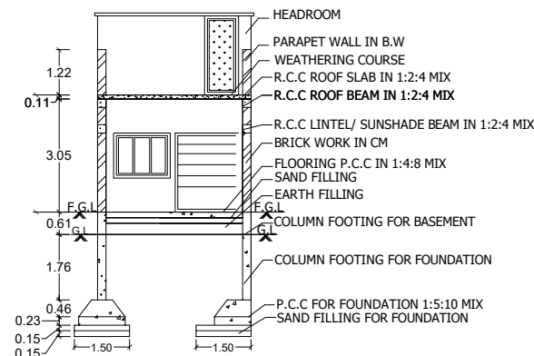
SECTION ON-AA
