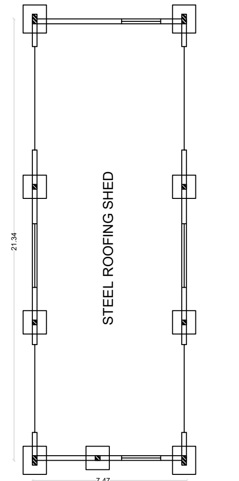
EXISTING SHED GROUND FLOOR
