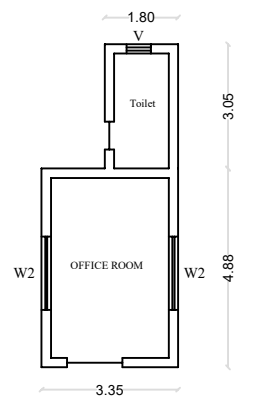
OFFICE BLOCK-1
