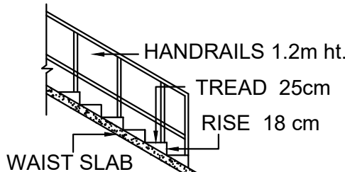
STAIRCASE DETAILS
