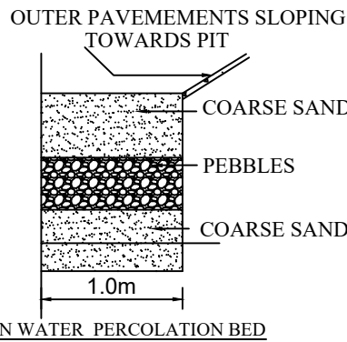
RAIN WATER PERCOLATION BED
