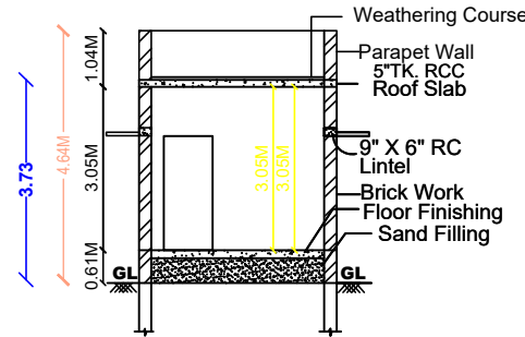
SECTION ON "BC"
