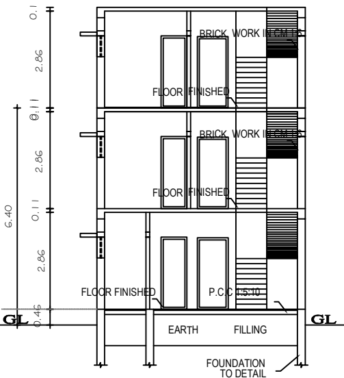
SECTION "A-B"
