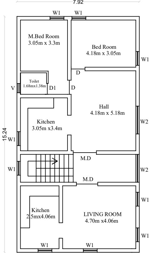
PRO. SECOND FLOOR PLAN.
