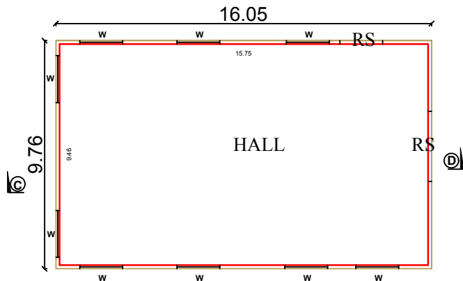
PRO.(MACHINARY HALL)
