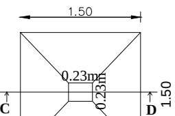
SECTION - 'CD'
