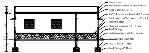
CROSS SECTION ON "AB"
