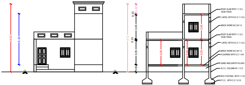
ELEVATION (NORTH FACING)
