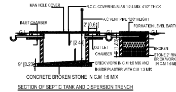
SECTION OF SEPTIC TANK AND DISPERSION TRENCH
