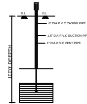
BORE WELL
