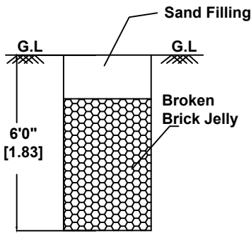
RAIN WATER HARVESTING RECHARGE PIT DETAILS (NOT TO SCALE)
