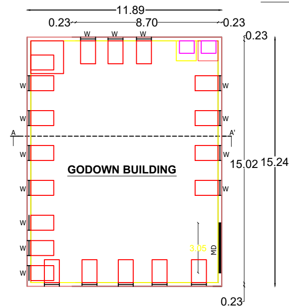
PROPOSED GROUND FLOOR PLAN FACING NORTH GODOWN BUILDING
