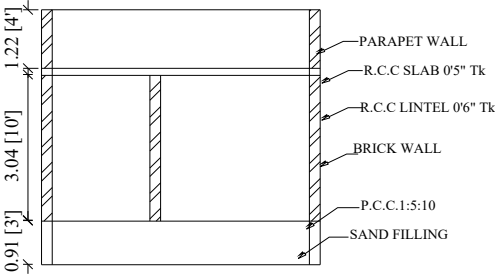
SECTION ON"AB"
