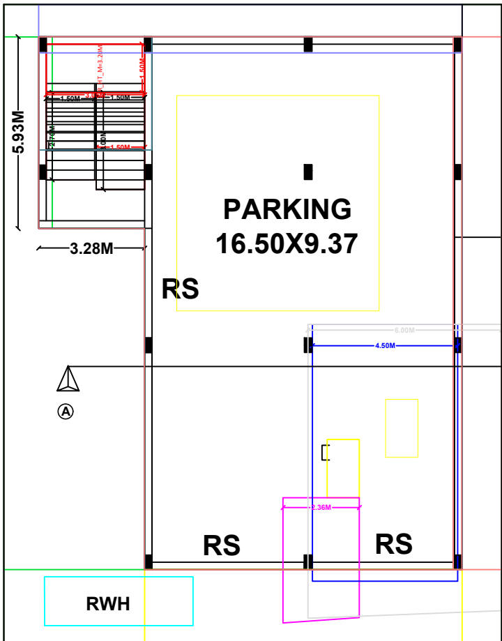
EX.STILT FLOOR PLAN
