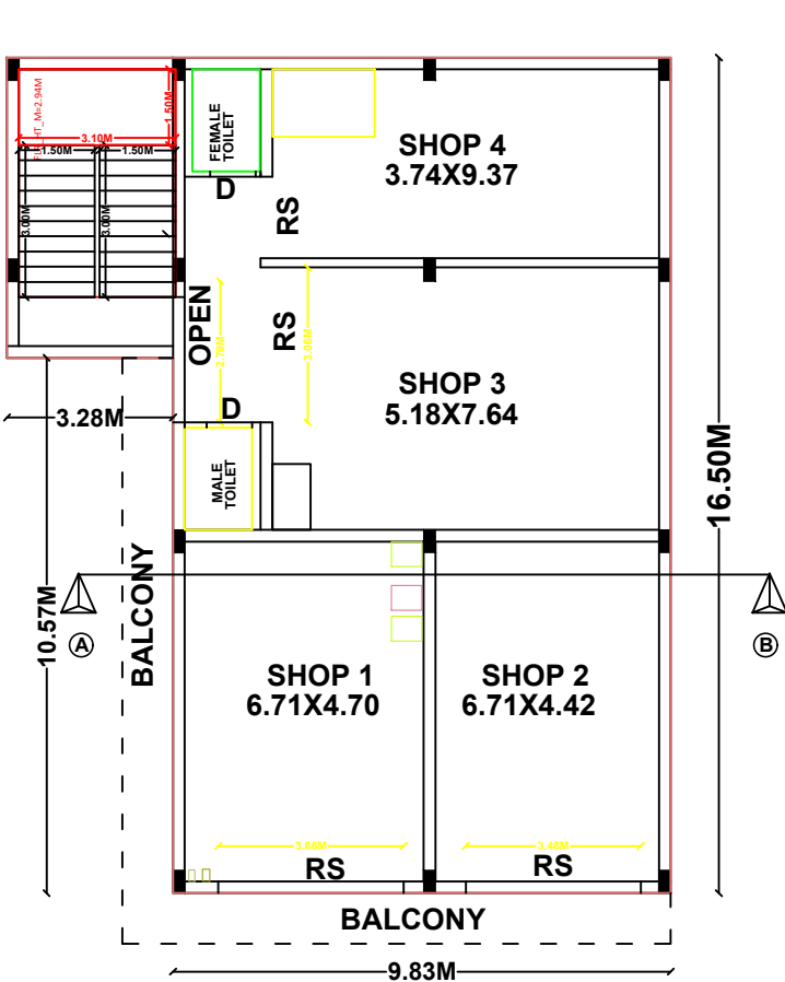
EX. GROUND FLOOR PLAN
