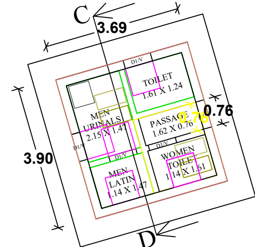
PLAN 2 - TOILET BLOCK
