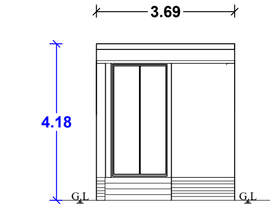
FRONT ELEVATION - 2
