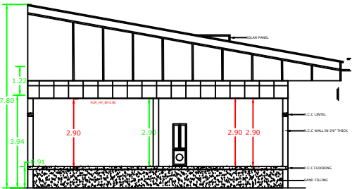
SECTION ON K-S
