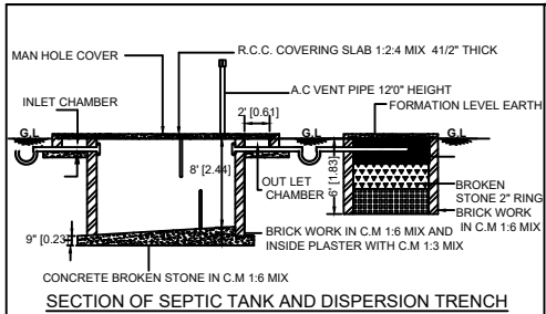
SECTION OF SEPTIC TANK AND DISPERSION TRENCH
