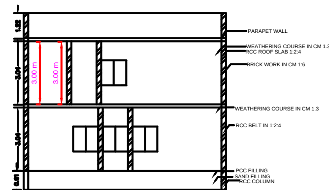
SECTIONON-"AA"&"BB"
