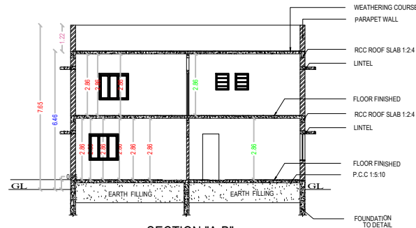
SECTION "A-B"
